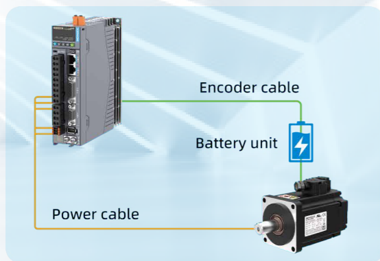
Encoder with battery
